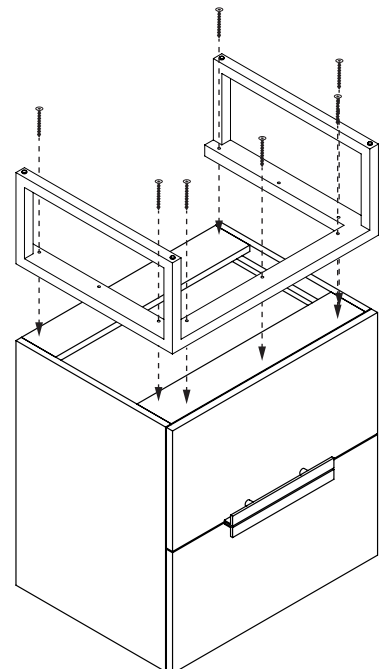
C-BASE INSTALLATION
